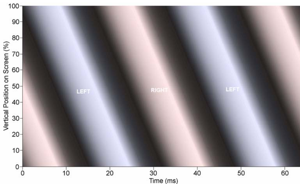
Figure 4: The spatial- and time-domain response of the example BFI LCD operating at 60Hz. The vertical axis shows the vertical position on the screen and the horizontal axis is time. The LEFT and RIGHT labels and tinting represent a sequence of left and right perspective images shown sequentially.
