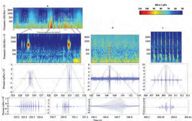
Figure 4. (a) Spectrogram of 4 days recording in Geographie Bay with a magnified spectrogram of 10 s at approximately 20:00 hrs on the 12th January, 2011. Waveforms of two recorded calls are shown with swimbladder pulses magnified. Circles in the top spectrogram highlight periods at dawn and dusk when similar calls were observed. (b) and (c) Spectrogram and waveform of unidentified calls recorded on 10th December 2010 at approximately 10:15 and 11:15 in Geographie Bay.
